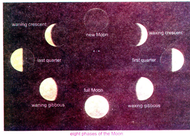
Figure: Phases of the Moon
